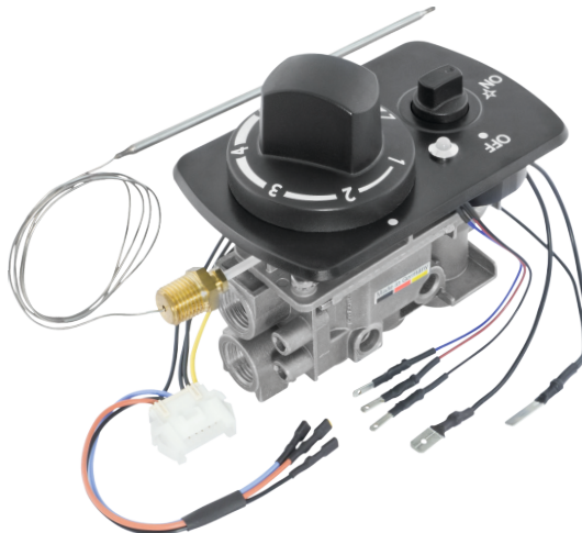
◀ GV30A thermostatic version with faceplate, large temperature knob and an electronic ignition module with LED pilot flame indication
