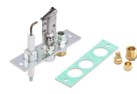
Pilot burner (G30-ZP2M-L, EU only) Sealing (G30-ZPS2) Pilot gas fitting (G30-ZPF...)
