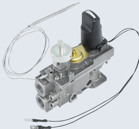
◀ GV30 with microswitch for electronic igniter
