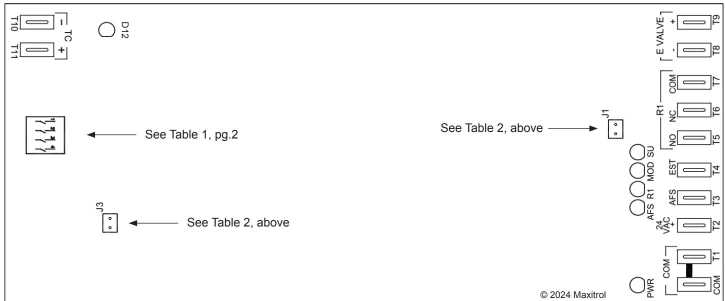
Figure 2: SC40 Trimpot, LED, Dip Switch and Jumper Locations
