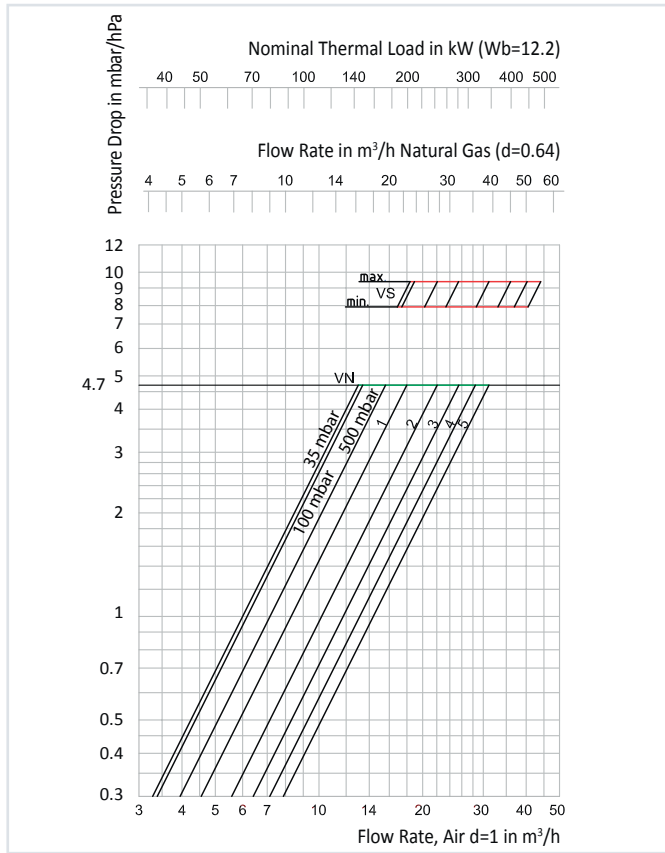
PRESSURE DROP SENTRY GS25 TYPE Z (35 mbar to 5 bar / 35 hPa to 0.5 MPa)
