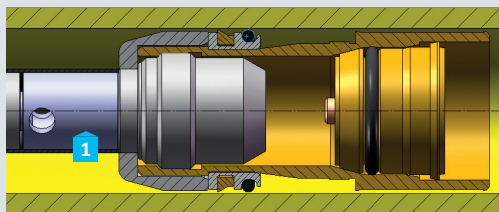
"In-pipe" EFV installation
