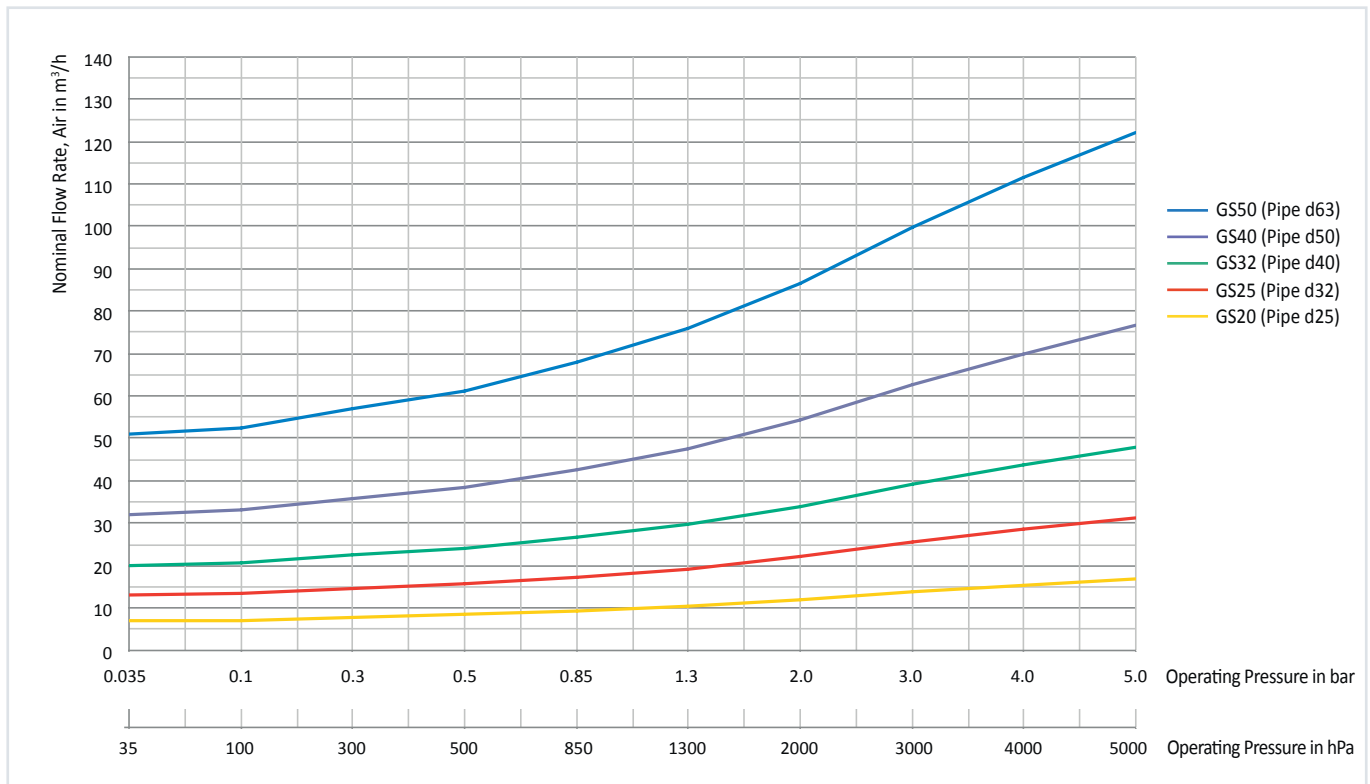
PRESSURE DEPENDENCE OF FLOW RATES SENTRY GS..Z
