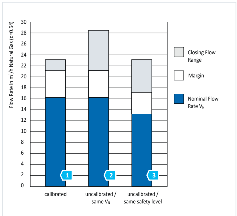
▼ Figure 4 Calibrated excess flow valves compared with uncalibrated. Example Maxitrol type Z in DN25
