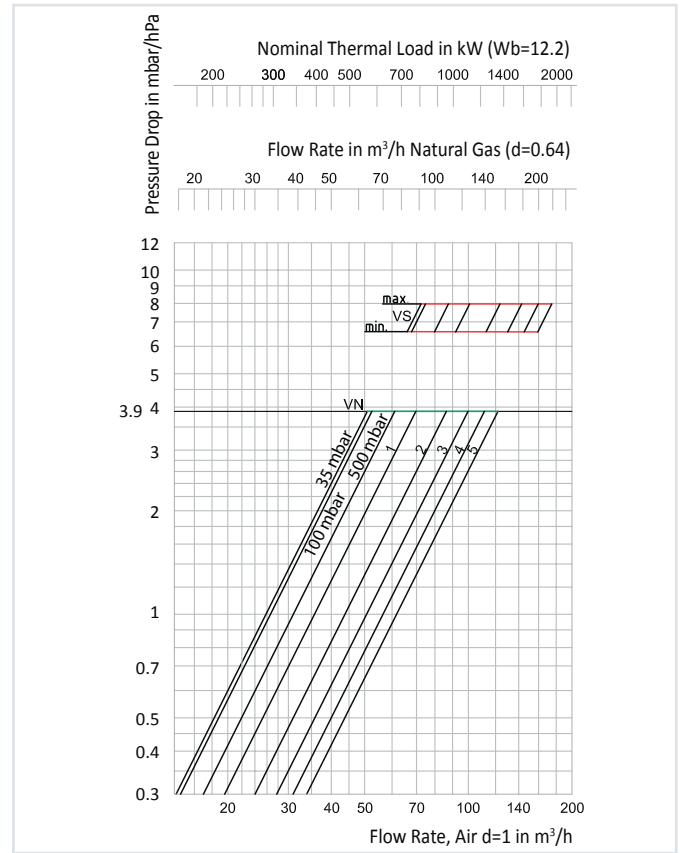
PRESSURE DROP SENTRY GS50 TYPE Z (35 mbar to 5 bar / 35 hPa to 0.5 MPa)
