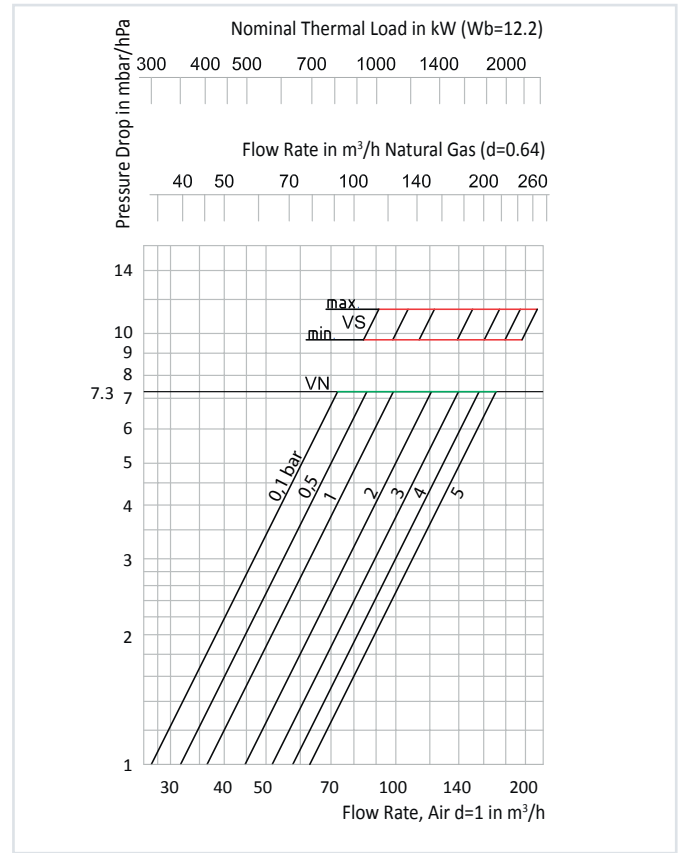
PRESSURE DROP SENTRY GS50 TYPE B (100 mbar to 5 bar / 100 hPa to 0.5 MPa)
