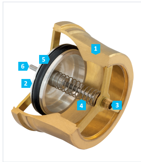
◀ Figure 1 Sectional view of a SENTRY GS in open position
