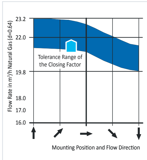
◀ Figure 3 Influence of mounting position on closing factor and tolerance. Example type Z in DN25
