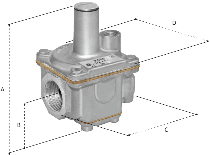
▲ R400S(M)...
