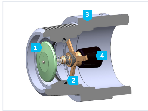
SENTRY GS cutaway (1" NPT)
